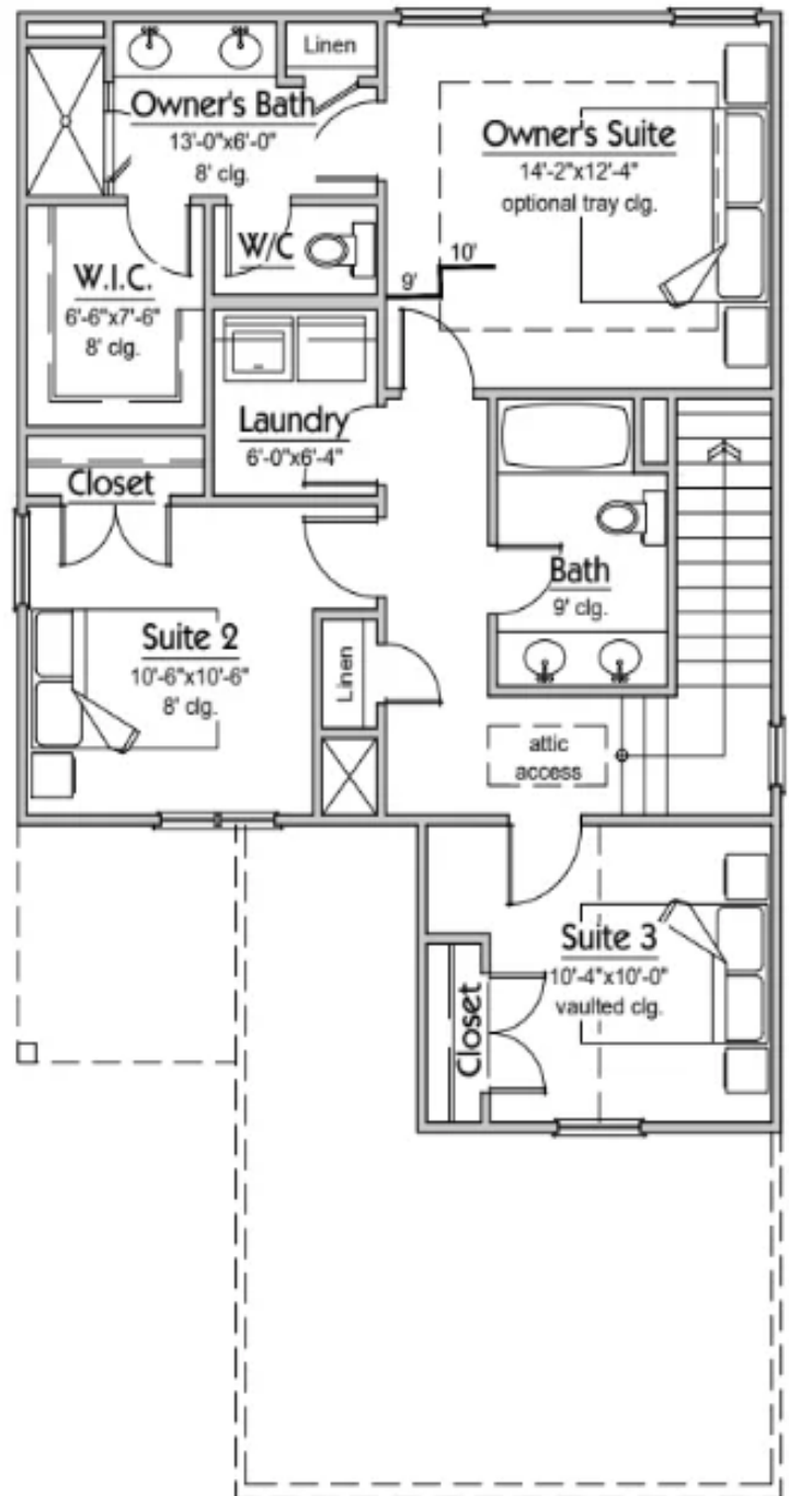
Upper Level Floor Plan
