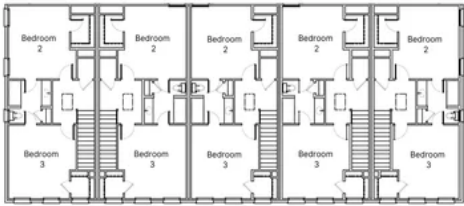
SECOND FLOOR
